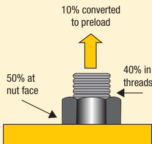
Frictional Losses (dry steel bolt)
