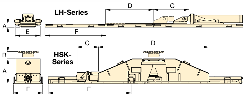
▼ Low-Height Skidding System assembly (LH400).
